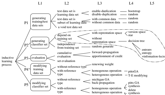
Fig. 1. The Hierarchy of Process Ontology
