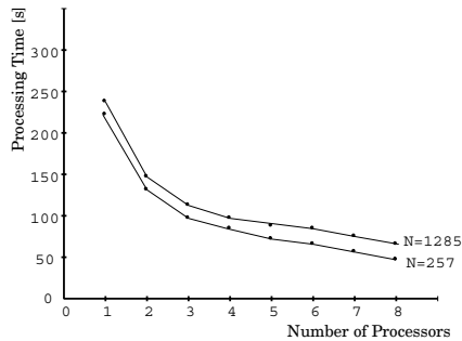
Fig. 2. Efficiency of the parallel algorithm.
