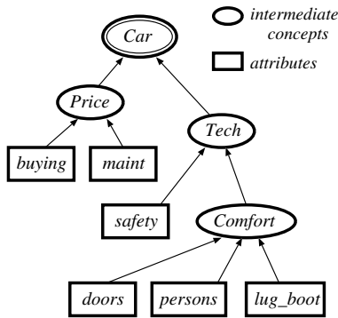
Fig. 1. The concept hierarchy
