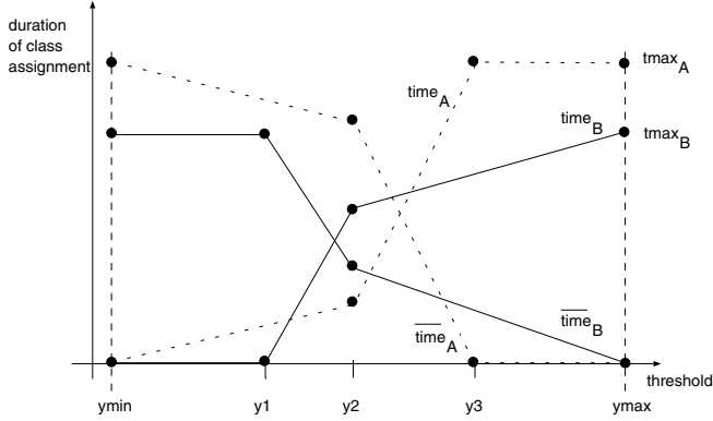
Fig. 2. Example of the function plots of the individual time_c and \overline{time}_c functions
