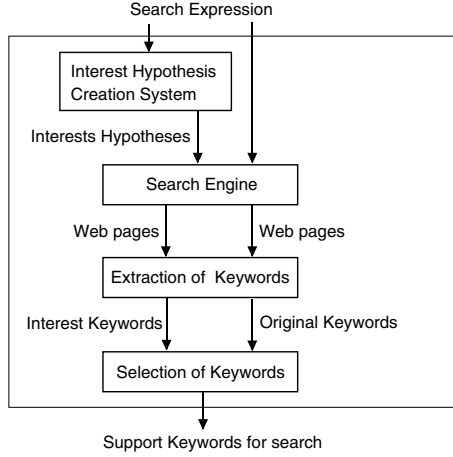
Fig. 4. Support System for User's Interests Expression
