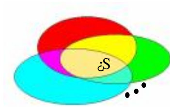
Fig.1. I = \cap_{k=1}^M S_k
