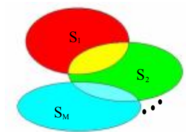
Fig.2. \cap_{k=1}^M S_k = \phi
