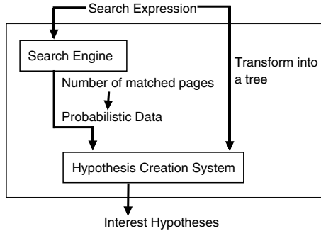
Fig. 1. Interest Hypotheses Discovering System
